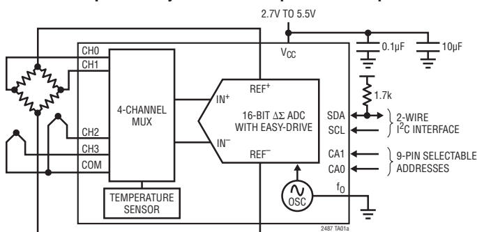
Data Acquisition System with Temperature Compensation
