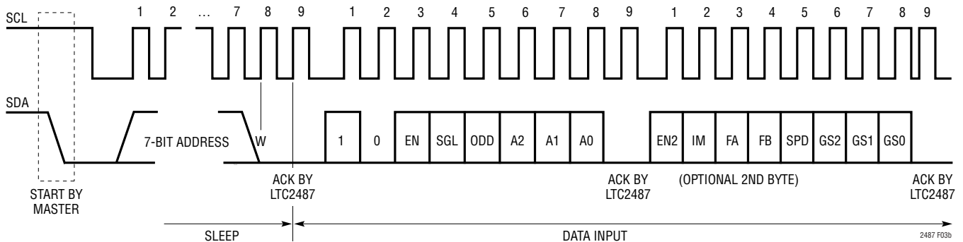
Figure 3b. Timing Diagram for Writing to the LTC2487
