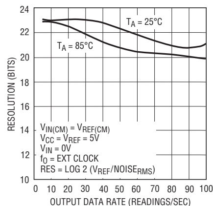
Figure 32. Resolution (Noise RMS ≤ 1LSB) vs Output Data Rate and Temperature
