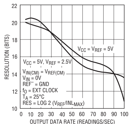
Figure 36. Resolution (INL MAX ≤ 1LSB) vs Output Data Rate and Temperature
