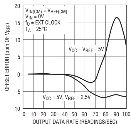
Figure 34. Offset Error vs Output Data Rate and Temperature
