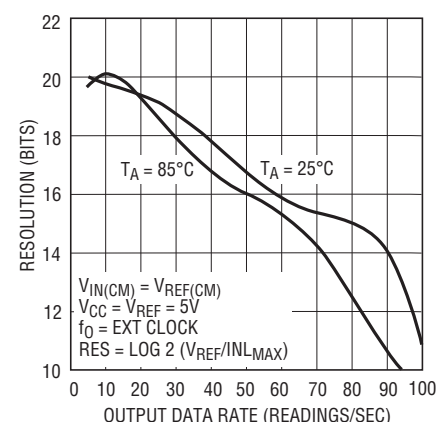
Figure 33. Resolution (INL MAX ≤ 1LSB) vs Output Data Rate and Temperature
