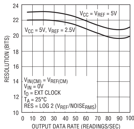
Figure 35. Resolution (Noise RMS ≤ 1LSB) vs Output Data Rate and Temperature
