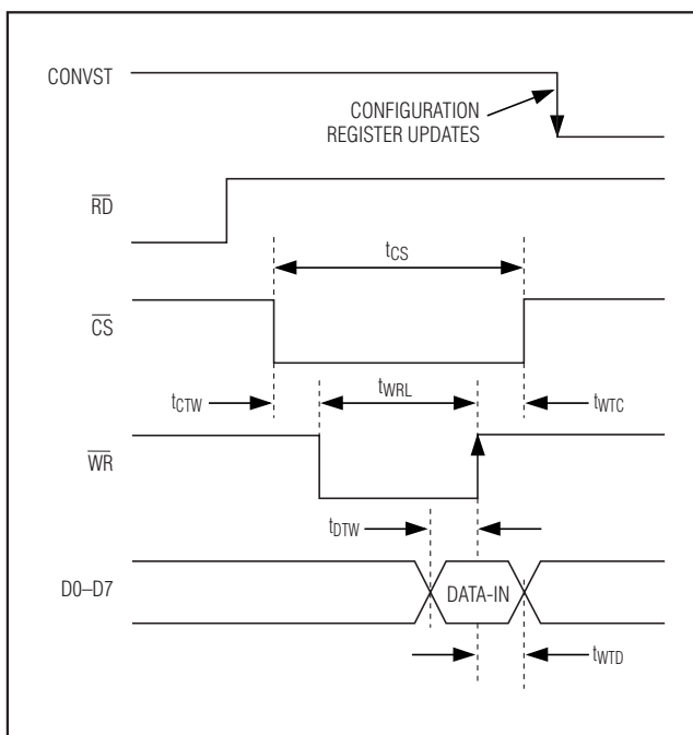
Figure 6. Write Timing
