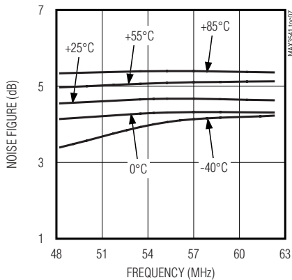
VHF NOISE FIGURE vs. FREQUENCY
