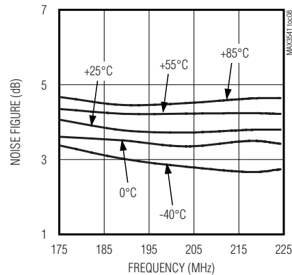
VHF NOISE FIGURE vs. FREQUENCY
