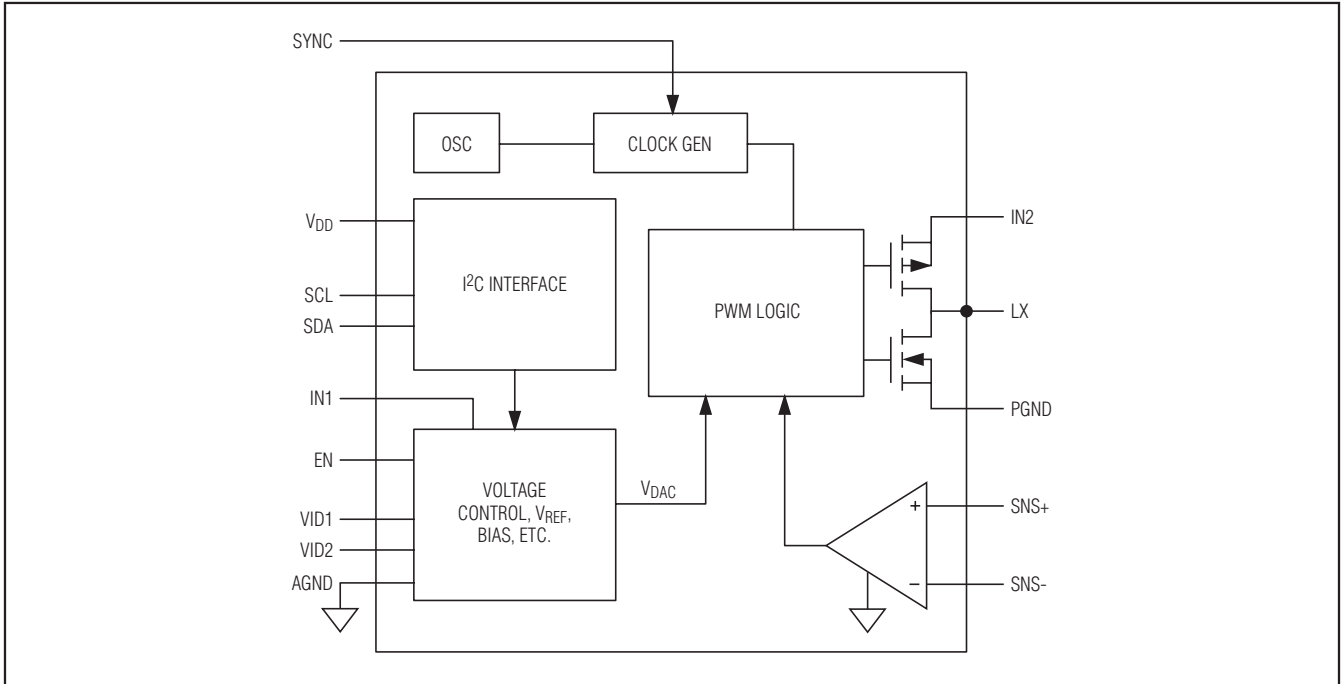
Figure 1. Block Diagram
