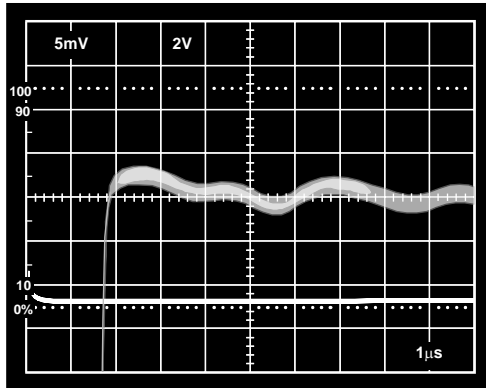
Figure 48. Positive Slope Settling Time
