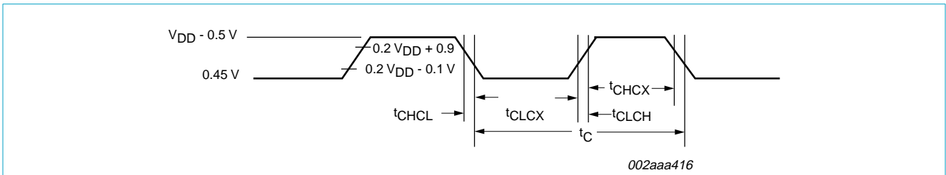
Fig 20. External clock timing.
