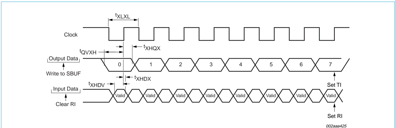
Fig 19. Shift register mode timing.
