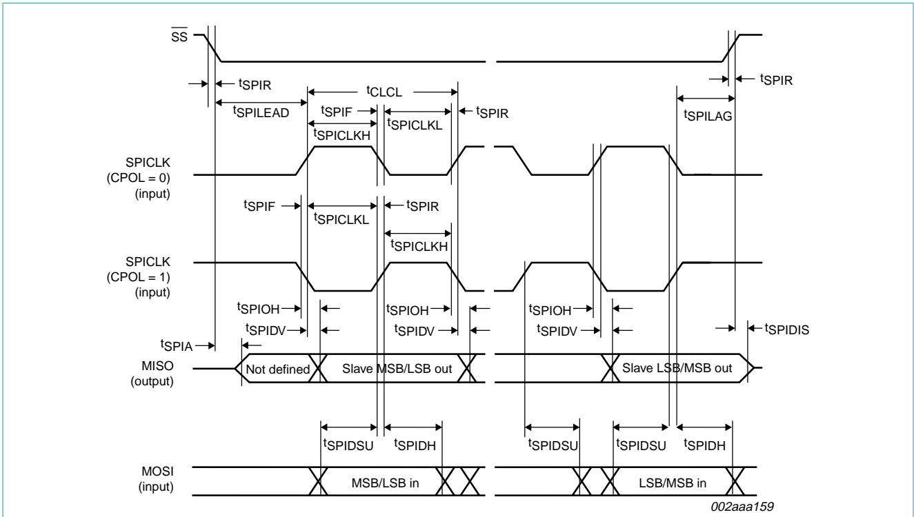
Fig 18. SPI slave timing (CPHA = 1).
