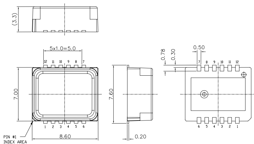
Figure 2. Housing dimensions
