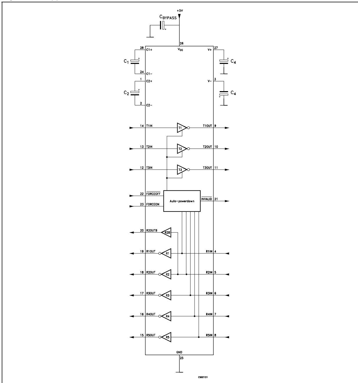
Figure 2. Application circuits
