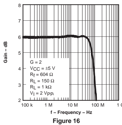
LARGE SIGNAL FREQUENCY RESPONSE
