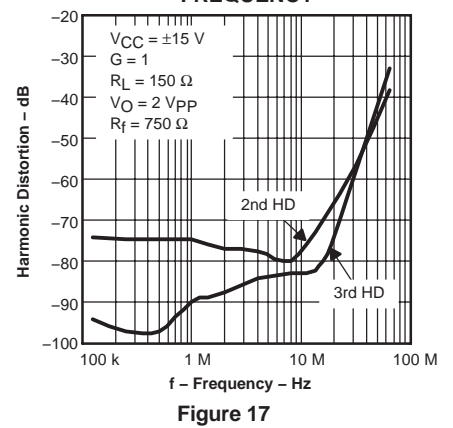
THS3061 HARMONIC DISTORTION VS FREQUENCY
