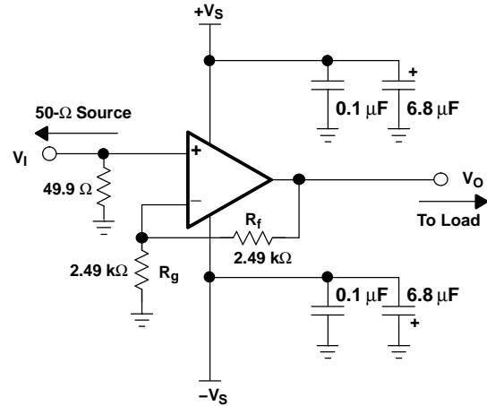
Figure 68. Wideband, Noninverting Gain Configuration
