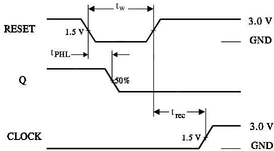
Figure 2. Switching Waveforms
