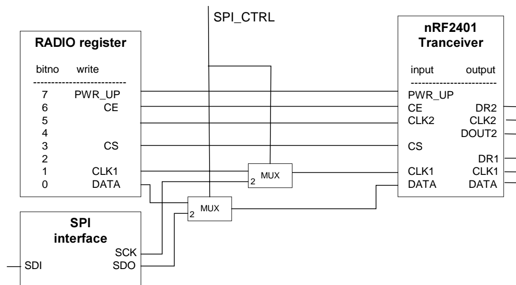
Figure 4-1 : Transmitter interface
