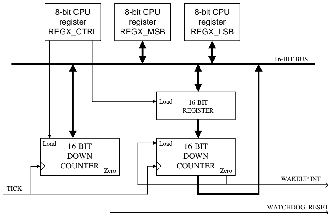
Figure 8-1 : RTC and watchdog block diagram
