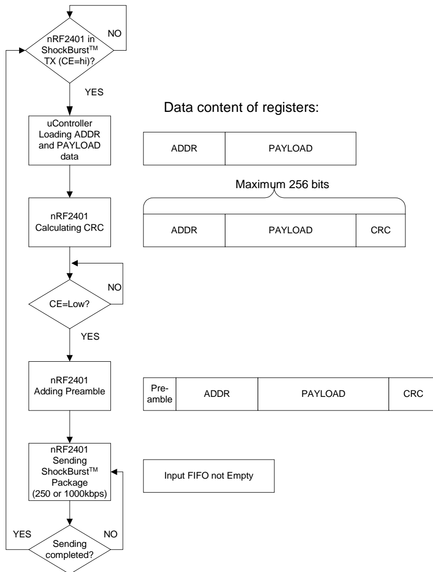
Figure 4-4 Flow Chart ShockBurst™ Transmit of transmitter subsystem
