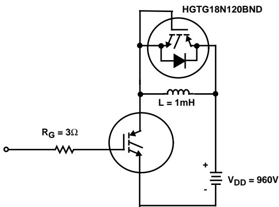
FIGURE 18. INDUCTIVE SWITCHING TEST CIRCUIT
