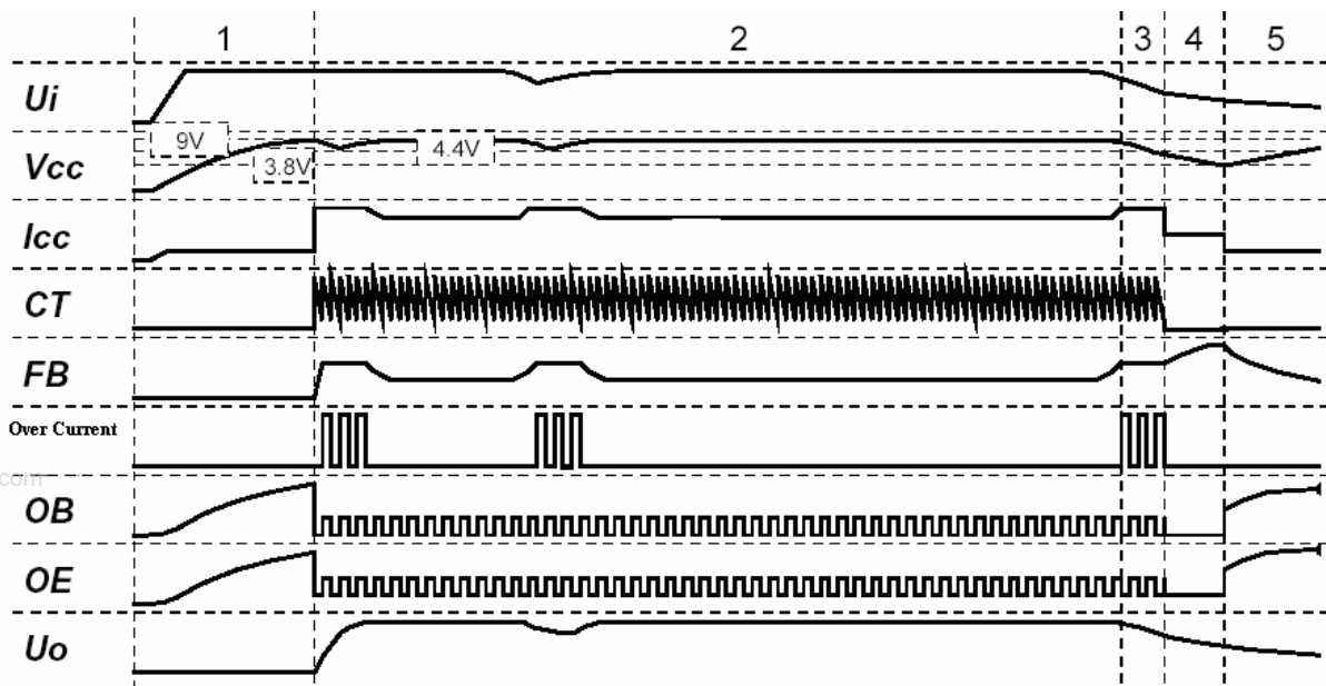
Fig.3 Overall Waveform Graph of THX203H
