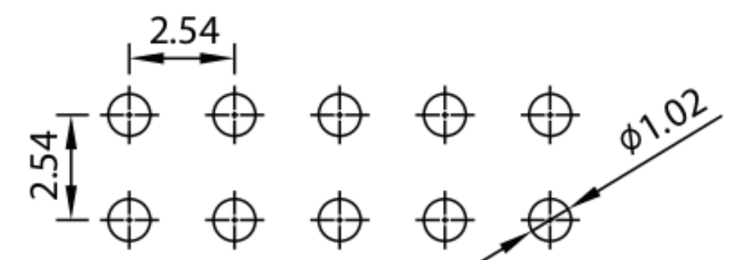
Recommended PCB Layout (PCB TOLERANCE \pm 0.05 )
