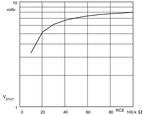
Fig. 7b V_{CEstat} as function of R_{CE}
