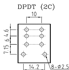
PC BOARD PATTEN (Bottom View)
