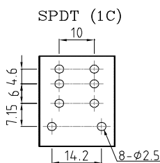
PC BOARD PATTEN (Bottom View)
