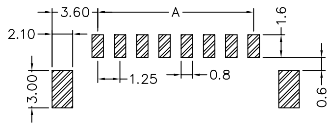
Recommended P.C.Board Pattern Dim.
