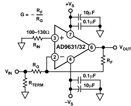
Figure 58. Inverting Operation
