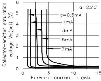
Fig. 11 Collector-emitter Saturation Voltage vs. Forward Current
