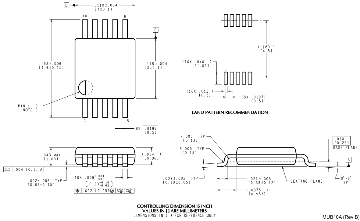
10-Pin MSOP NS Package Number MUB10A
