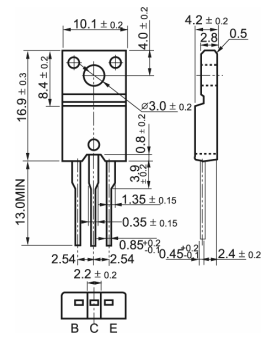
TO-220F
