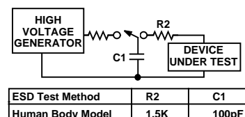
Figure 21. ESD Generator
