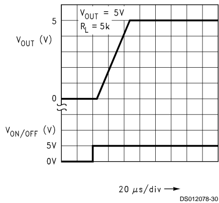
Turn-On Waveform
