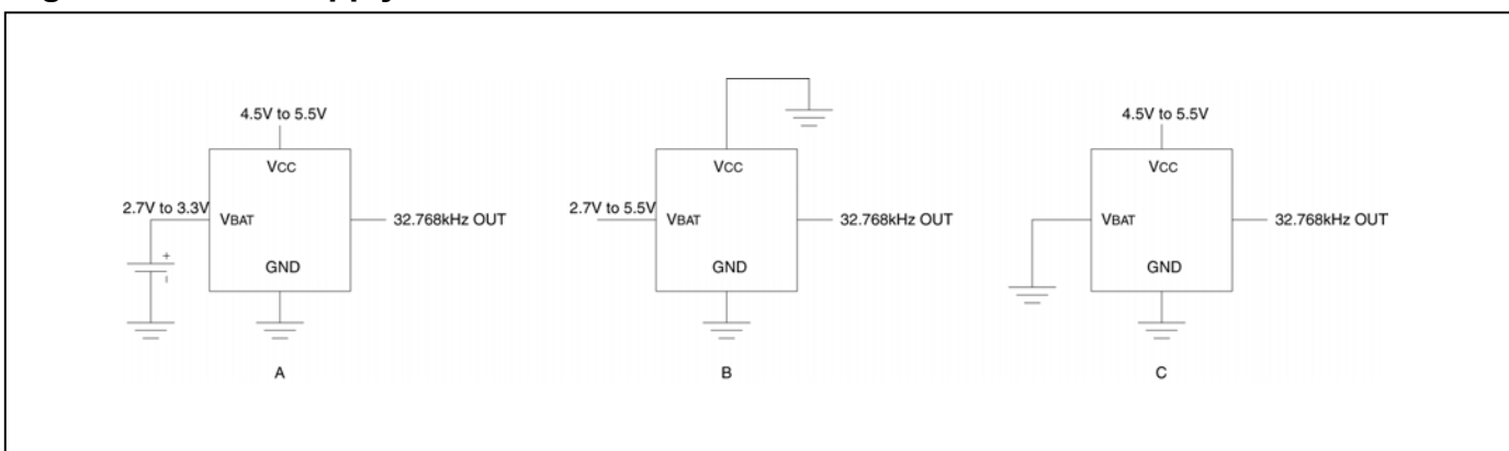
Figure 3. Power-Supply Connections
