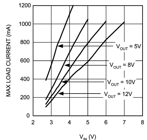
Max. Load Current (typ) vs V_{\text{IN}} - "Y"
