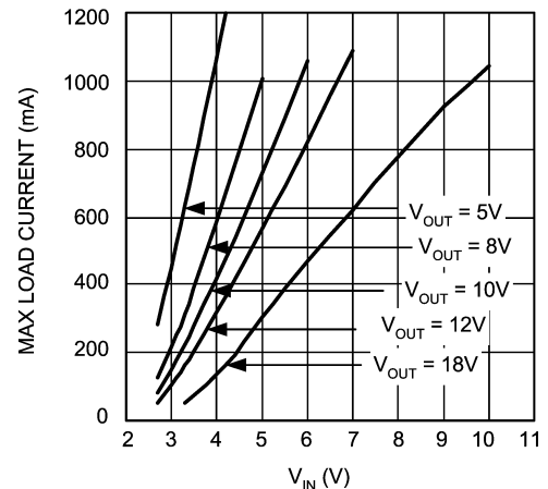
Max. Load Current (typ) vs V_{\text{IN}} - "X"
