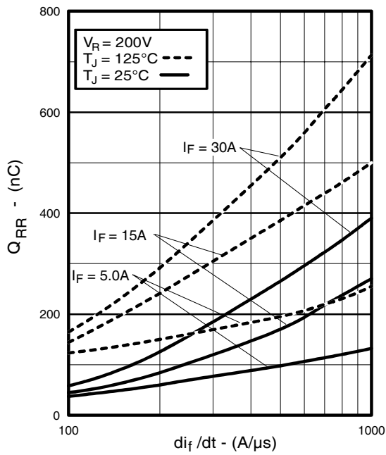
Fig. 21 - Typical Stored Charge vs. di/dt
