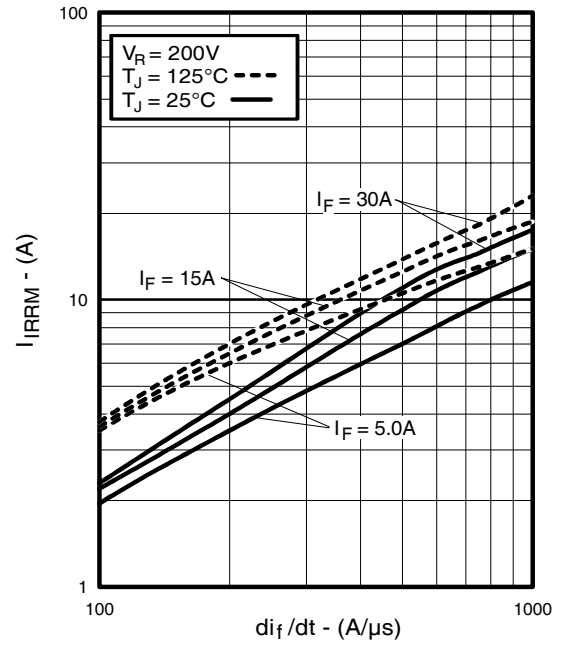
Fig. 20 - Typical Recovery Current vs. di/dt
