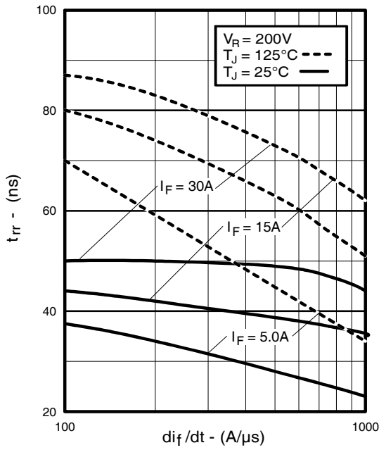
Fig. 19 - Typical Reverse Recovery vs. di/dt
