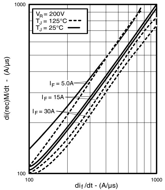
Fig. 22 - Typical di_{(rec)M}/dt vs. di/dt
