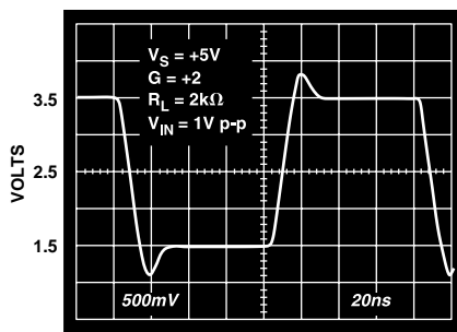
Figure 32. Large Signal Step Response; V_S = +5 \text{ V} , G = +2
