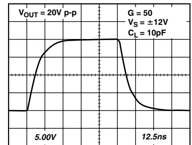
TPC 108. AD8129 Transient Response, V_{OUT} = 20\text{ V p-p} , G = 50 , V_S = \pm 12\text{ V}
