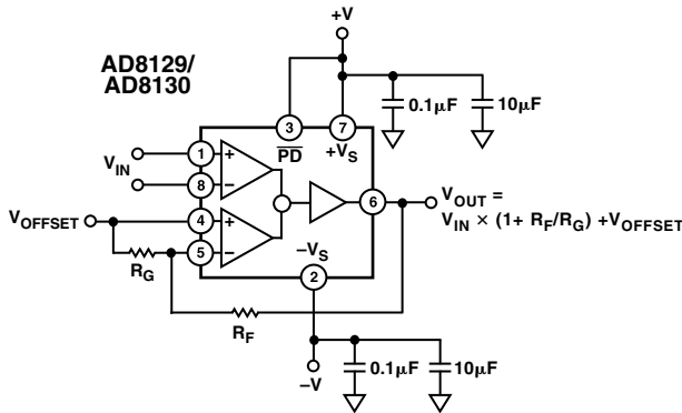
Figure 12. In this circuit, V_{OFFSET} appears at the output with unity gain. This circuit works well if the V_{OFFSET} Source Impedance is low.
