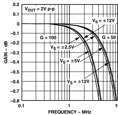
TPC 32. AD8129 Fine Scale Response vs. Supply, G = 50 , G = 100 , V_{OUT} = 2 V p-p
