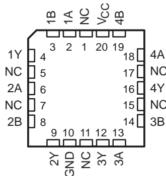
SN54HC132 . . . FK PACKAGE (TOP VIEW)
