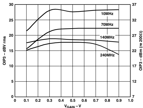
TPC 6. OIP3 vs. V_{GAIN}
