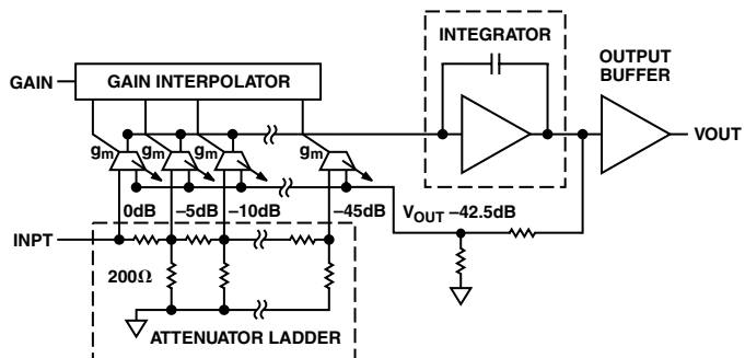
Figure 1. The Simplified Architecture
