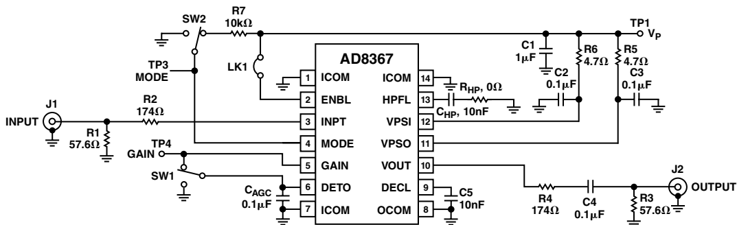
Figure 16. Evaluation Board Schematic
