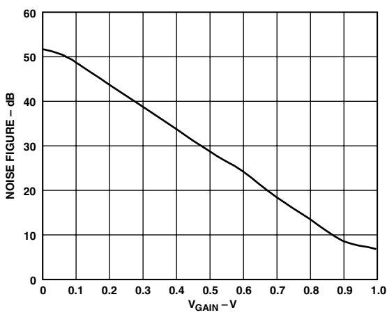
TPC 5. NF (re 200 \Omega ) vs. V_{GAIN} at 70 MHz
