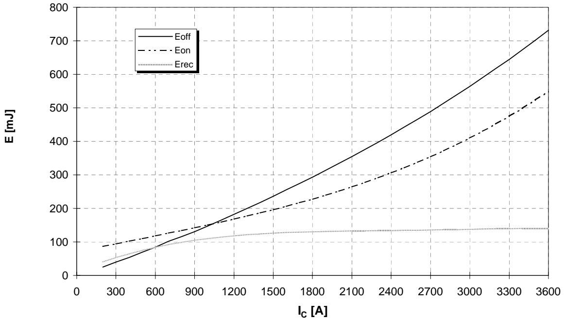
Schaltverluste (typisch) E_{on} = f(I_C) , E_{off} = f(I_C) , E_{rec} = f(I_C) Switching losses (typical) R_{gon} = R_{goff} = 0,51 \Omega , V_{CE} = 600V , T_j = 125^\circ C
