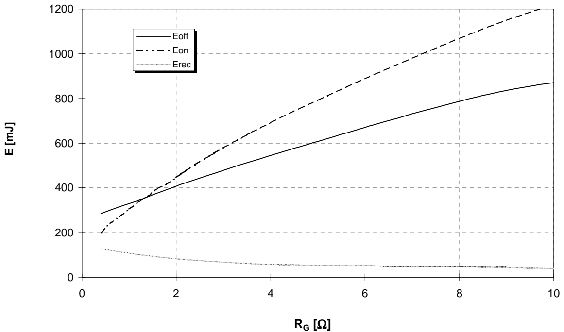
Schaltverluste (typisch) E_{on} = f(R_G) , E_{off} = f(R_G) , E_{rec} = f(R_G) Switching losses (typical) I_C = 1800A , V_{CE} = 600V , T_j = 125^\circ C
