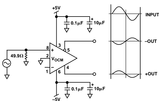
Figure 41. Unity Gain, Single-Ended-to-Differential Amplifier
