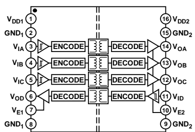
Figure 2. ADuM1401
