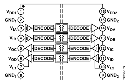
Figure 3. ADuM1402
