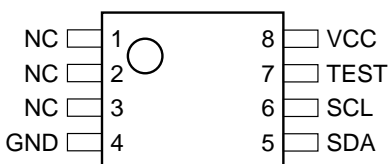
8-Pin TSSOP
