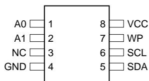
8-lead SOIC
