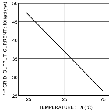
Fig.7 "H" grid output current temperature characteristics
