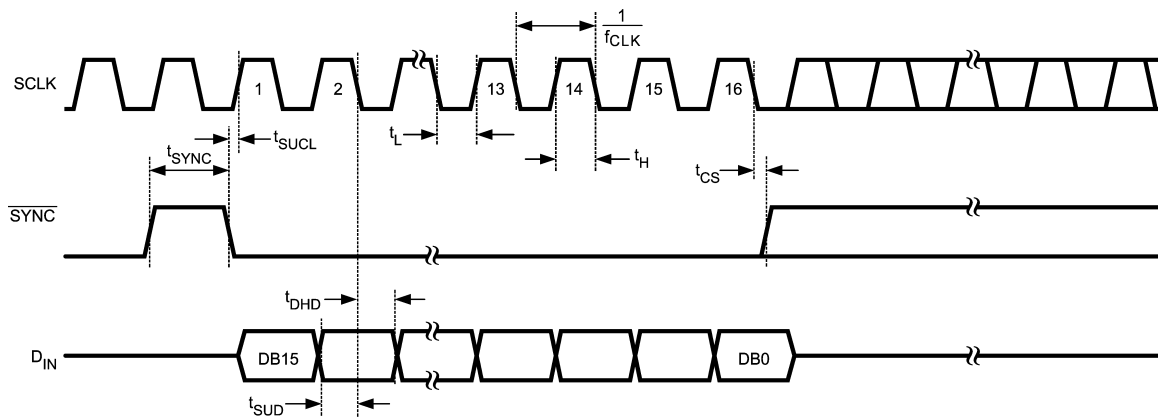
FIGURE 2. DAC081S101 Timing
