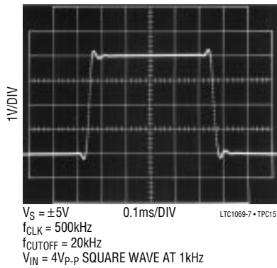
Transient Response
