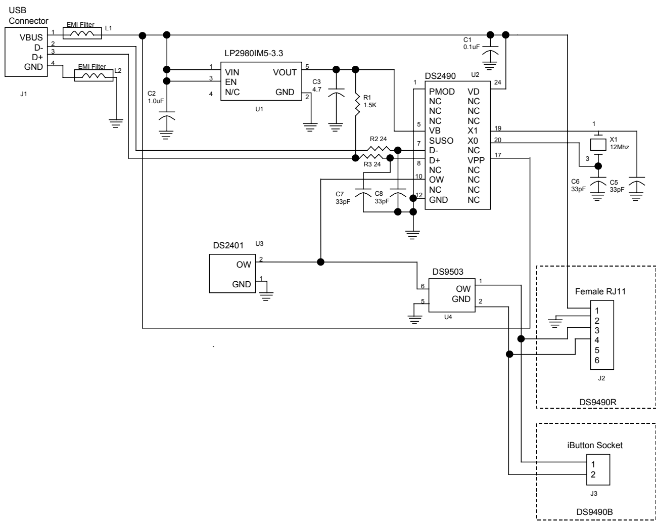
Figure 8. FUNCTIONAL DIAGRAM
