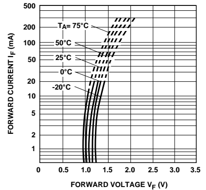
Figure 13. Typical Forward Current vs. Forward Voltage, HCPL-3100.
