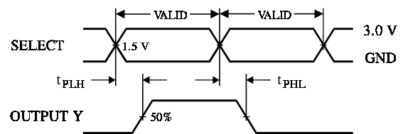
Figure 2. Switching Waveforms
