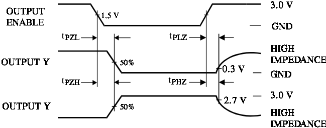
Figure 3. Switching Waveforms
