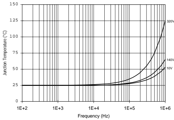
Figure 28. IR2112 T J vs. Frequency (IRFBC20) R GATE = 33Ω, V CC = 15V
