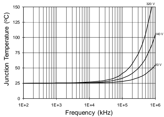
Figure 28. IRS2110/IRS2113 T_J vs. Frequency (IRFBC20) R_{GATE} = 33 \text{ W} , V_{CC} = 15 \text{ V}
