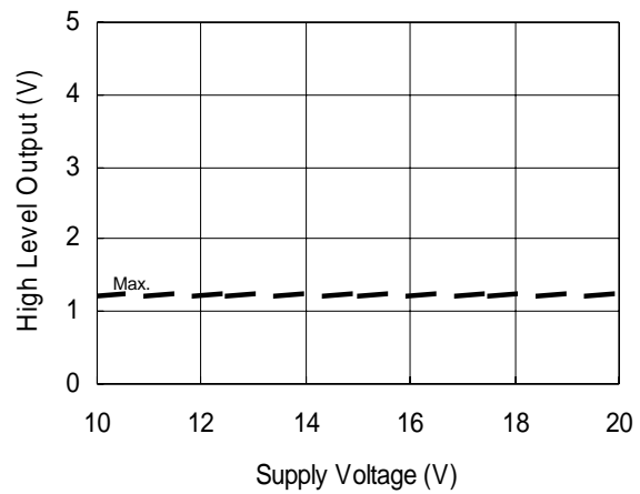
Figure 10B. High Level Output vs. Supply Voltage
