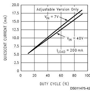
Quiescent Current vs Duty Cycle
