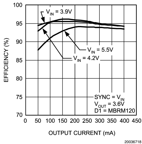
Efficiency vs Output Current ( V_{OUT} = 3.6V , PWM MODE, with Diode)
