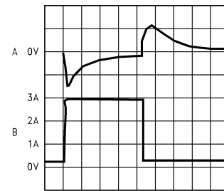
200 \mu sec/Div DS100886-20
