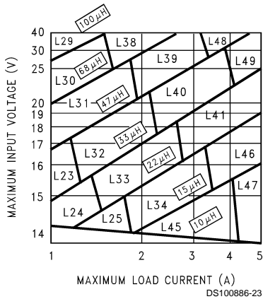
FIGURE 5. LM2678-12
