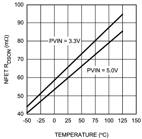
NMOS Switch R_{DSON} vs Temperature and PVIN
